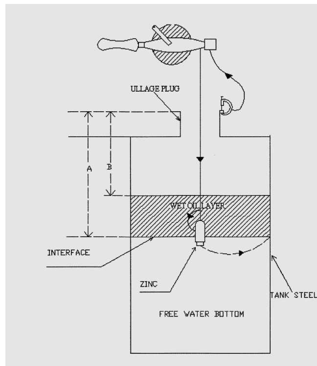
Figure 5 (A) Oil/water interface detector
