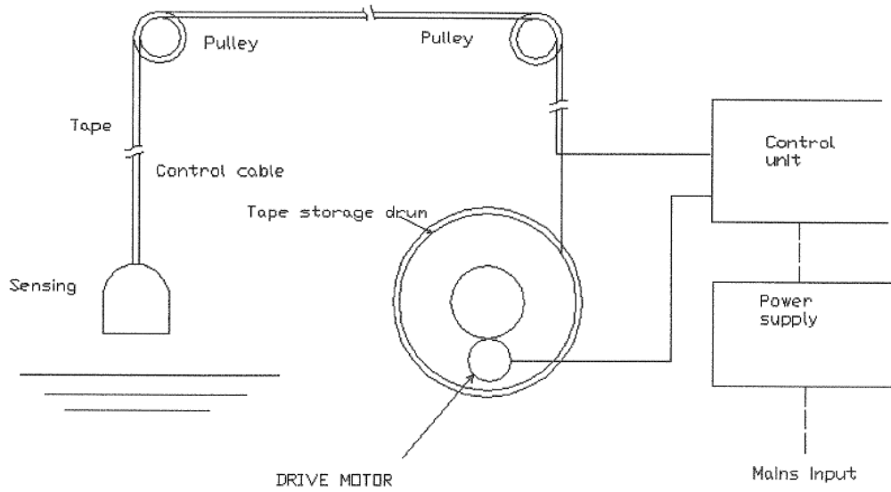
Figure 1 (J) Electrically powered servo-operated gauge
