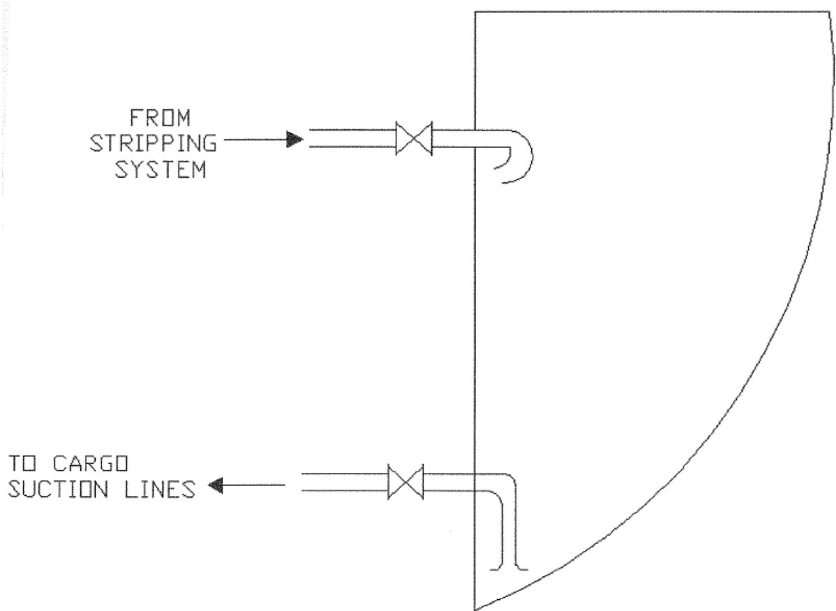
Figure 1 (F) Slop – tank arrangement
