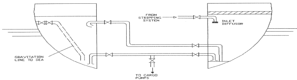
Figure 1 (G) Efficient slop-tank arrangement
